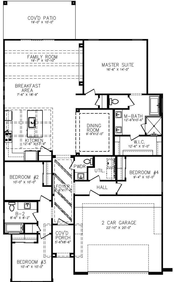
FLOOR PLAN
