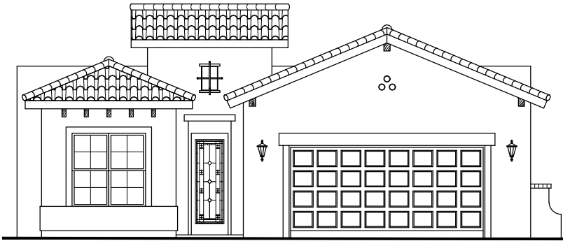
FRONT ELEVATION
