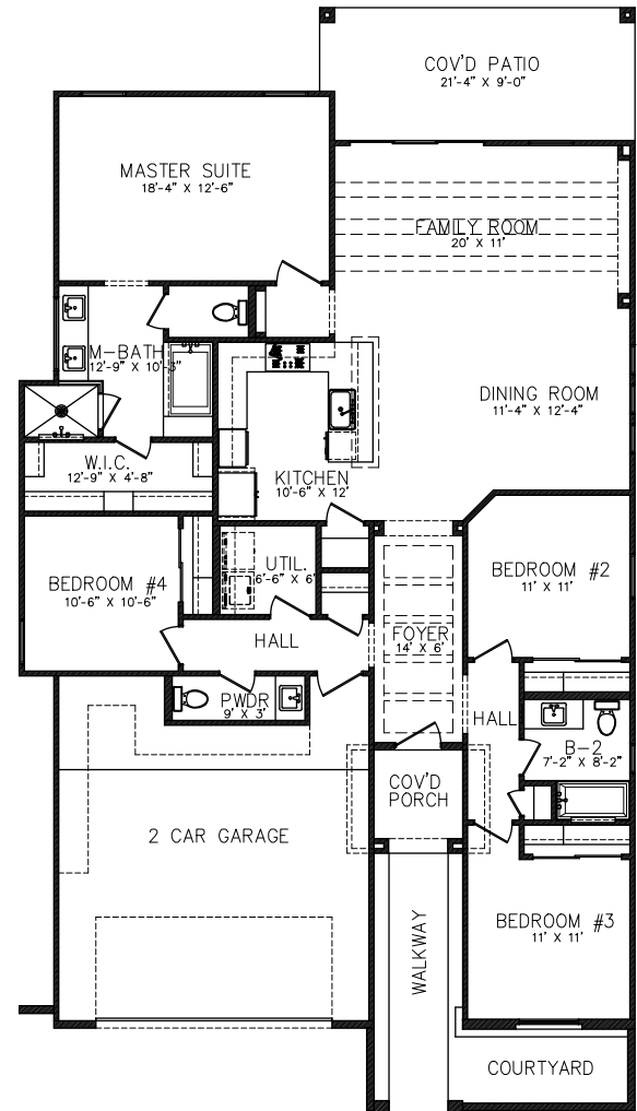
FLOOR PLAN
