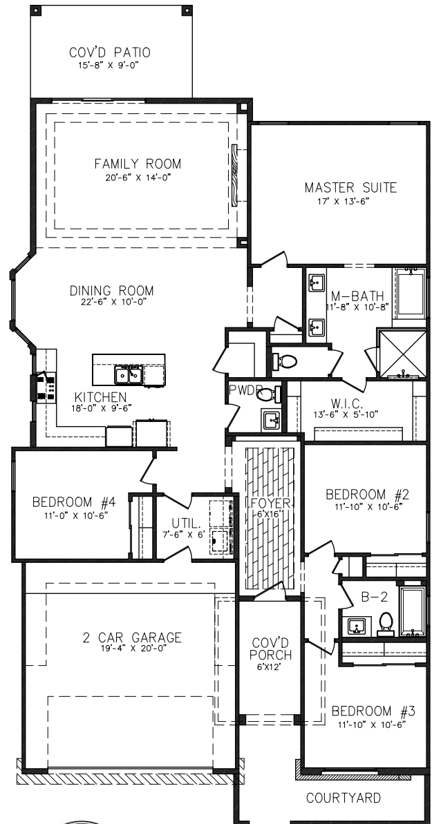
FLOOR PLAN
