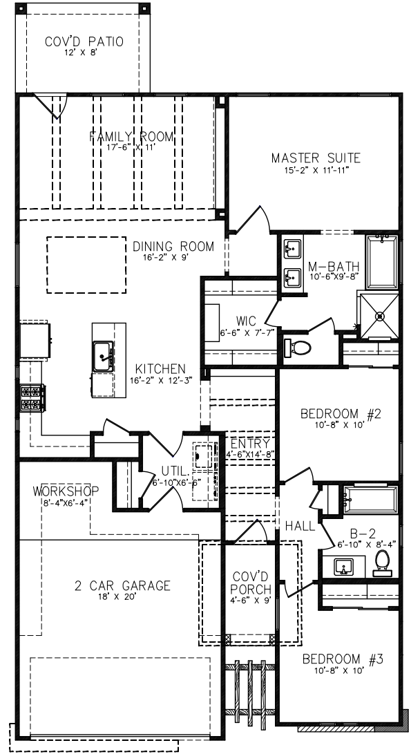
FLOOR PLAN
