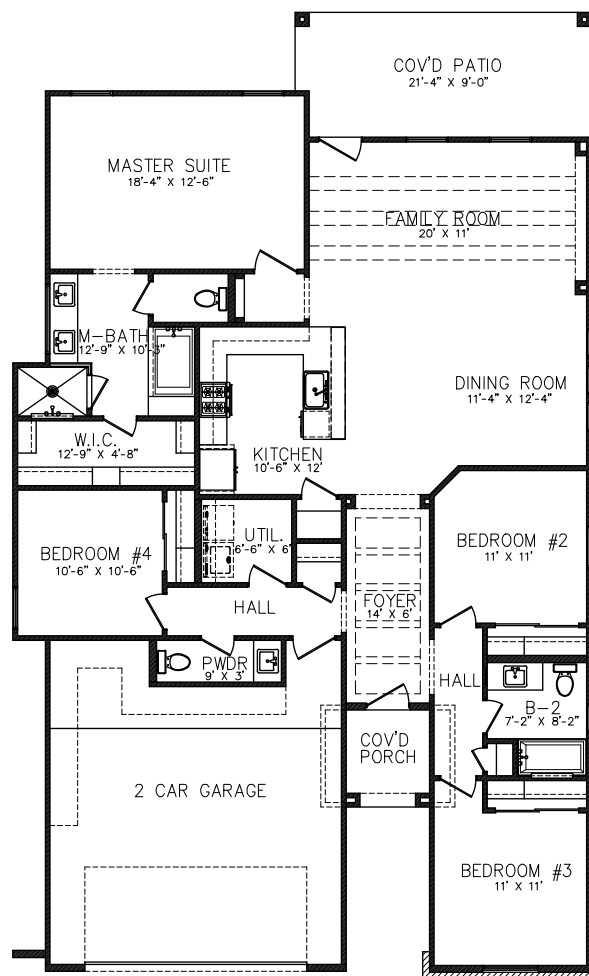
FLOOR PLAN
