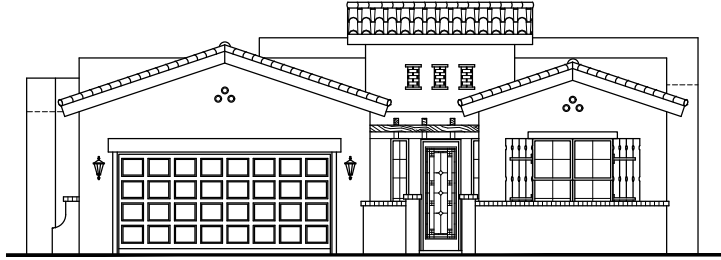
ELEVATION "A"
