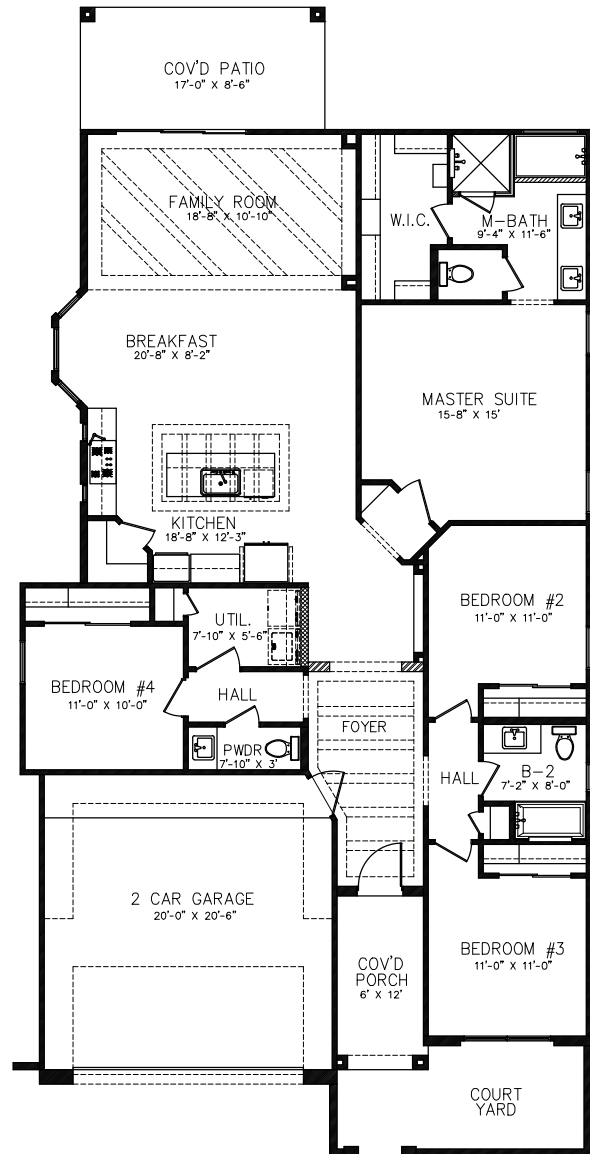
FLOOR PLAN
