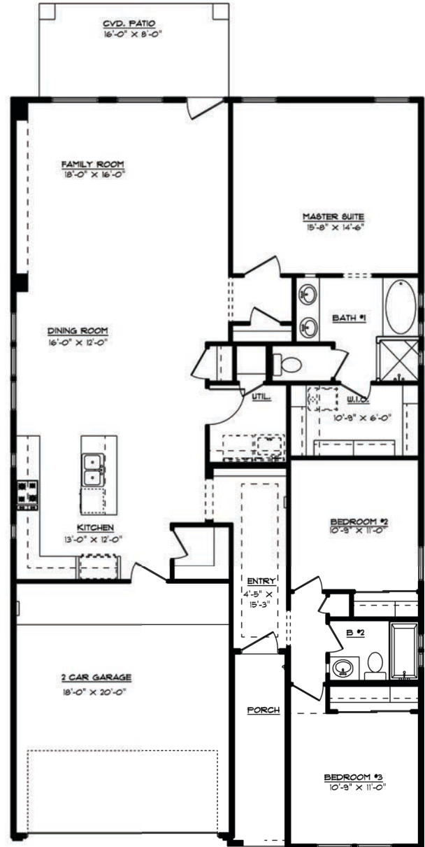
FLOOR PLAN
